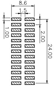
SMT P.C.Board Layout (TOLERANCE = ±0.05)
